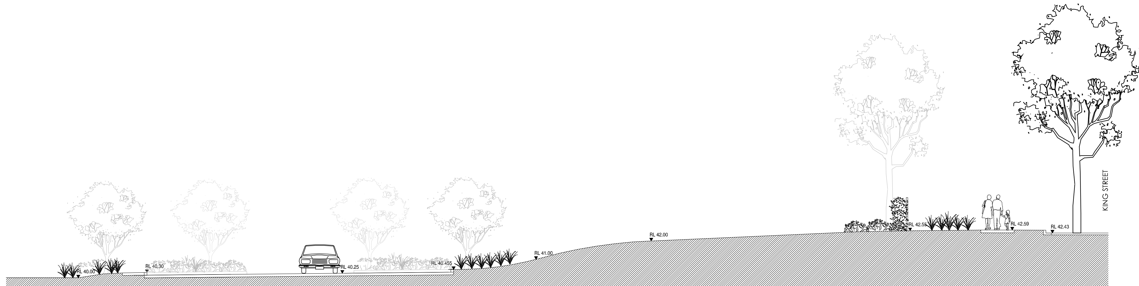
2 SECTION A SECTION 1:100
